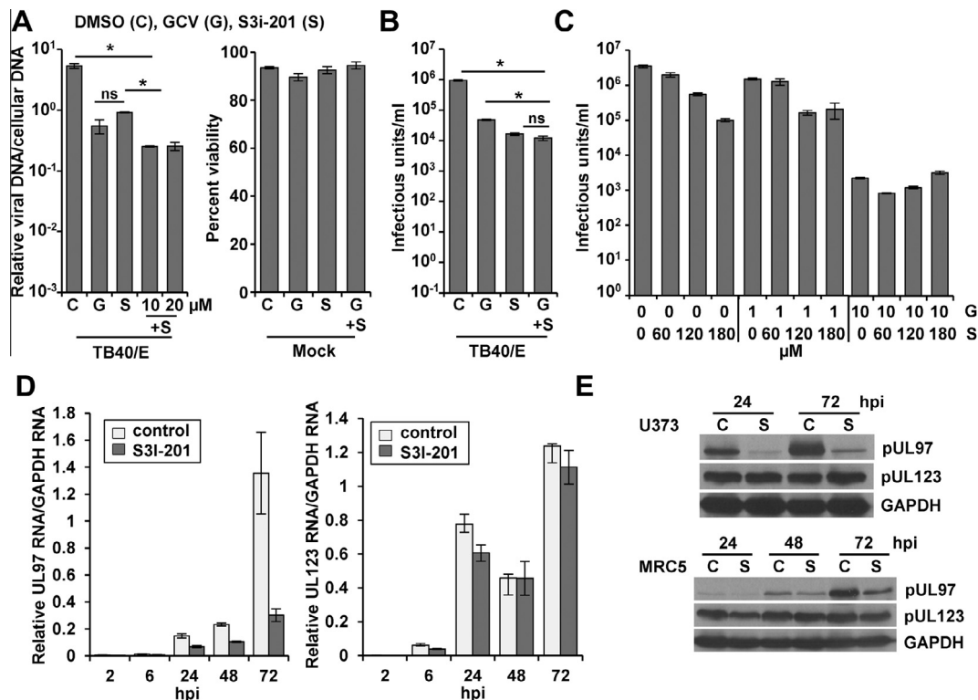
Fig. 3. S3i-201 treatment decreases UL97 expression. (A) Fibroblasts were pretreated with 100 \mu M S3i-201 (S) or DMSO (C). After 24 h, cells were infected at 3 IU/cell with either ADwt virus or TB40/E virus. Cells were treated with 10 or 20 \mu M GCV (G) and S3i-201 at the time of infection. At 72 hpi, viral genomes were quantified by qPCR and normalized to cellular DNA. Cell viability of uninfected cells was quantified using flow cytometry at 72 hpi. Data represent the mean of two replicate experiments \pm SEM. (B) Fibroblasts treated as above using 10 \mu M GCV and infected at 3 IU/cell using TB40/E virus. Viral titers were determined from culture supernatants obtained at 96 hpi. Data represent the mean of four replicates \pm SEM. (C) Fibroblasts were pretreated with different concentrations of S3i-201 with DMSO and then treated with 1 or 10 \mu M GCV upon infection. Cells were infected and analyzed as described above. Data represent the mean of two replicates \pm SEM. (D) U373 cells were pretreated with DMSO or 100 \mu M S3i-201. After 24 h, cells were infected at 0.25 IU/cell with TB40/E virus. Expression of RNAs was quantified by qRT-PCR. Data represents the mean of two replicate experiments \pm SEM. (E) U373 cells and MRC5 fibroblasts were pretreated with S3i-201, infected as described above, and analyzed by Western blot. (* p < 0.05).
