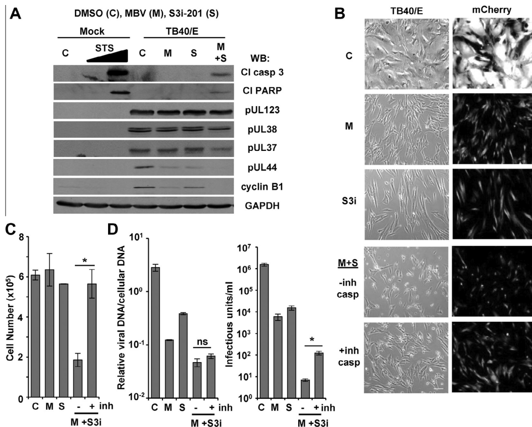
Fig. 4. Caspase-dependent loss of infected cells upon inhibition of both STAT3 and pUL97. (A) MRC-5 fibroblasts were pretreated with 100 \mu M S3i-201 (S) or DMSO (C). After 24 h, cells were infected at 5 IU/cell using TB40/E virus. Cells were treated with 40 \mu M MBV (M) or MBV and S3i-201 at the time of infection and harvested at 48 hpi. Mock infected cells were treated with 0, 0.5, or 1.0 \mu M staurosporine (STS) for 3 h prior to Western blot analysis using the indicated antibodies. (B) MRC-5 fibroblasts were treated and infected as described above. At 48 hpi, cells treated with MBV and S3i-201 were treated with 50 \mu M of Z-VAD and Z-DEVD-FMK or DMSO control. At 72 hpi, live cells were imaged for viral infection (TB40/E expressing mCherry) and cell morphology (brightfield) using fluorescence microscopy. (C) MRC-5 fibroblasts were treated and infected as described above. At 48 hpi, cells treated with MBV and S3i-201 were treated with 50 \mu M of Z-VAD and Z-DEVD-FMK. At 72 hpi, adherent cells were harvested and total cell number was quantified using flow cytometry. Data represent the mean of three replicates \pm SEM. (D) Fibroblasts were treated as described above. At 72 hpi, viral genomes were quantified by qPCR and normalized to cellular DNA (left panel). Viral titers were determined from culture supernatants obtained at 96 hpi (right panel). Data represent the mean of four replicates \pm SEM. (* p < 0.05 ).
