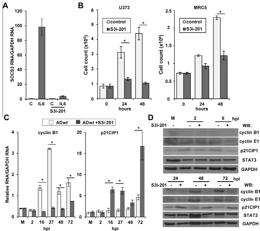
Fig. 1. Chemical inhibition of STAT3 activity decreases cellular proliferation. (A) U373 cells were pretreated with DMSO or 125 \mu M S3i-201. After 24 h, cells were treated with DMSO or recombinant human IL-6 for 45 min. SOCS3 RNA was quantified by qRT-PCR. Data represents the mean of two replicate experiments \pm SEM. (B) U373 and MRC-5 cells were seeded subconfluent. After 24 h, U373 were treated with DMSO or 60 \mu M S3i-201 while fibroblasts were treated with 100 \mu M S3i-201. Total cell number was determined at the indicated times post drug treatment. (C) U373 cells were pretreated with DMSO or 125 \mu M S3i-201. After 24 h, cells were infected at 0.25 IU/cell using ADwt virus. Expression of RNAs was quantified by qRT-PCR. Data represents the mean of two replicate experiments \pm SEM. (D) U373 cells were pretreated with drug and infected as described above. Western blot was completed using the indicated antibodies. (* p < 0.05 ).
